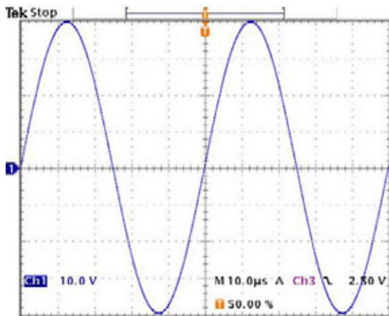
80Vp-p 20kHz into 4Ω load, G=-10, Cc=100pF
