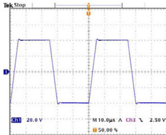
20kHz square response, 80Vp-p, 4Ω load, G=-10, Cc=100pF
