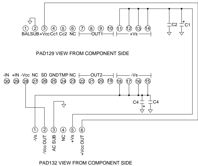
FIGURE 3. IMPLEMENTING RAIL TO RAIL OPERATION USING PAD130 ACCESSORY MODULE
